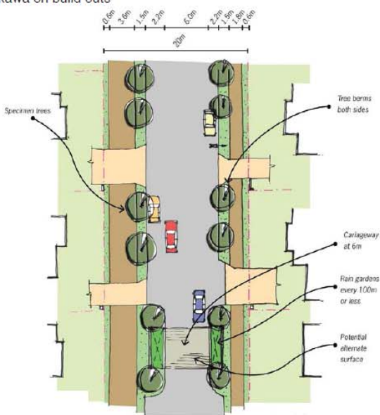
Figure 16 - Planting Guide - Ihumatao Quarry Road - Stage 1
